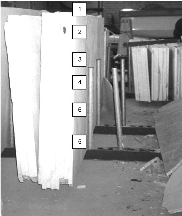
Picture 6.4 – Example of too little clearance angle with too large overall thickness of the slab.
